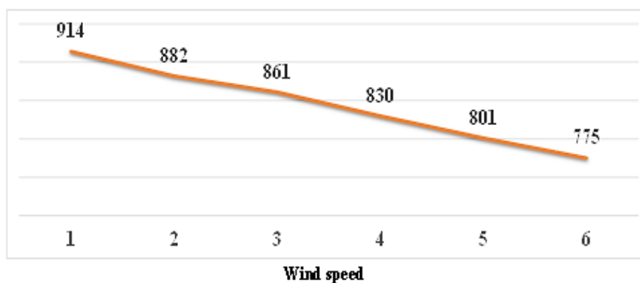
Fig. 7. Total flight time depending on wind speed changes.
